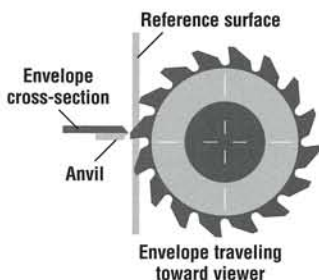
Ovation's unique milling cutter produces a soft, feathered edge.
